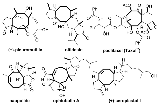
Scheme 1. Natural products containing cyclooctane rings.
